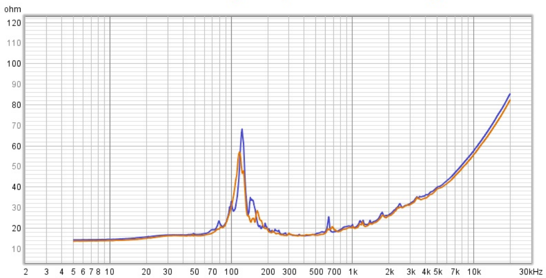
Marshall 4x12 16R (G12M) AX=Blue BX=Orange
